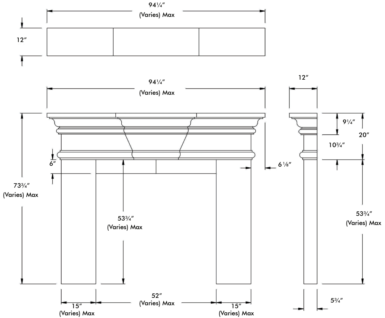
FRONT ELEVATION
